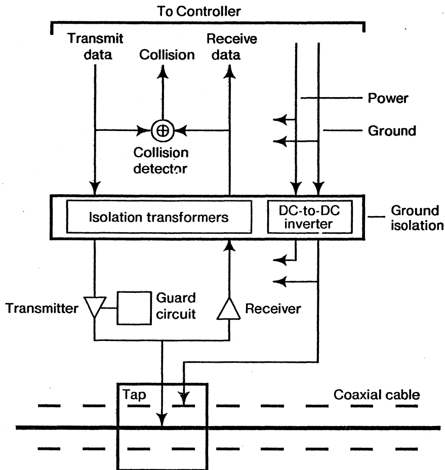
Figure 3. Ethernet Transceiver
