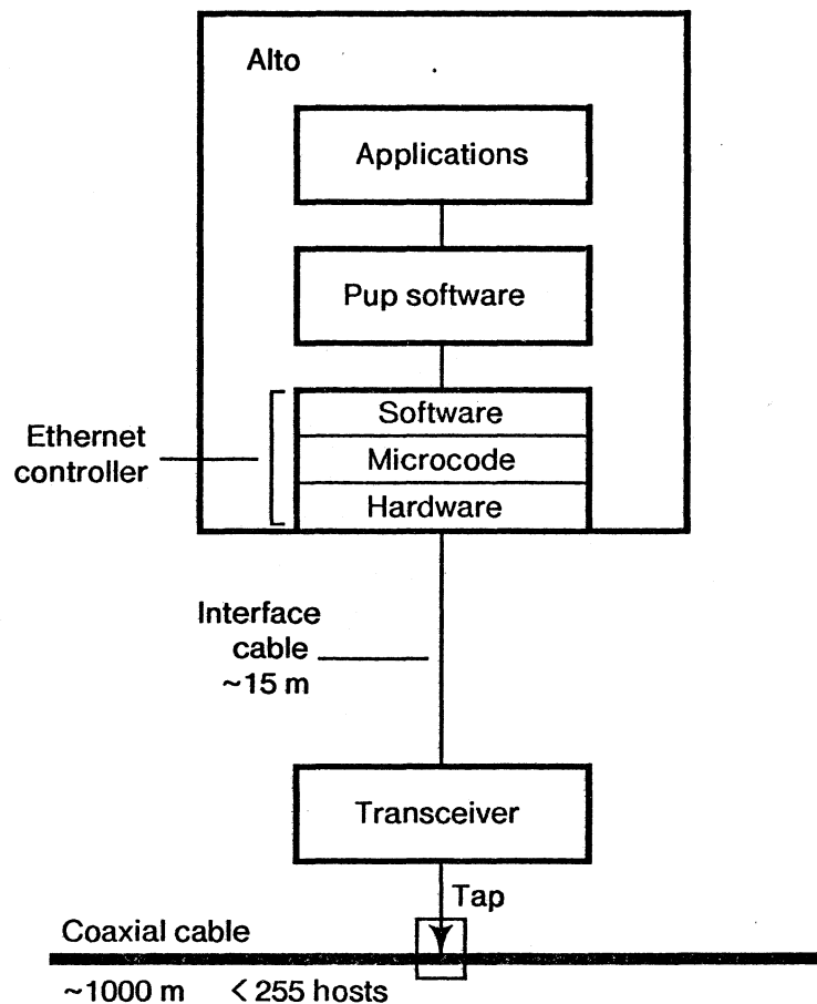
Figure 2. Alto-Ethernet connection
